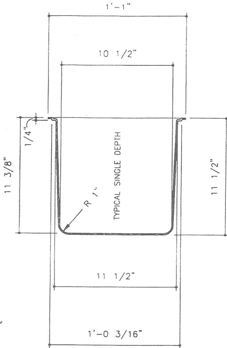
SGL. DEPTH LINER DETAIL (11-1/2" squared at the opening)
